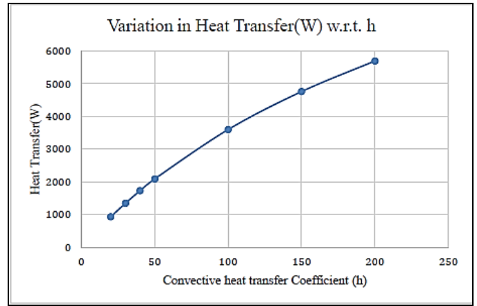
Fig.4 Effect of h on rate of heat transfer
