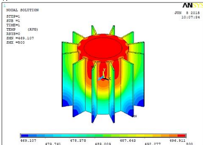
Fig.3 Temperature Profile across Parallel fin -24 No configuration
