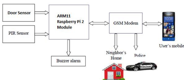
Fig. Block diagram of In-home Security System
