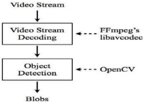
Fig. shows the simplified diagram of this detection process. FFmpeg is used only to decode the video stream. Then, the object detection function uses the decoded data to detect any moving object by using the available programming interfaces provided by Open CV. We have presented video motion detection methods, motion vector (MV) based and, using open source tools, FFmpeg and OpenCV libraries. With the existing tools, we could build moving object detection application by simply extending the video decoding functions .
