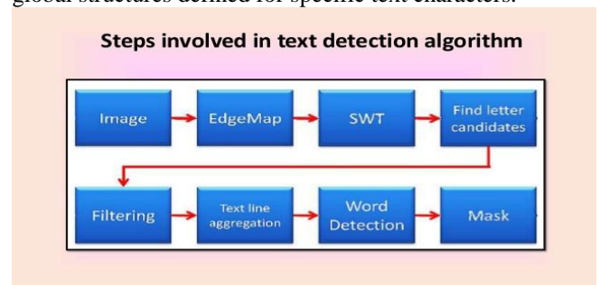
Fig. text detection algorithm.
