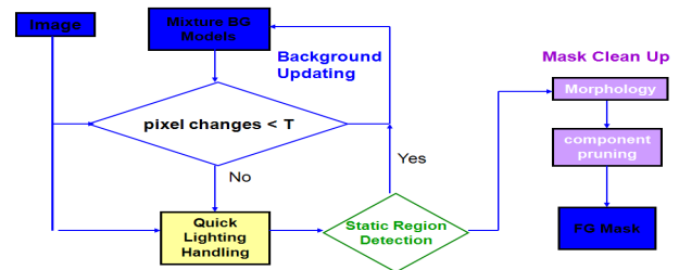
Fig. Background subtraction method.
