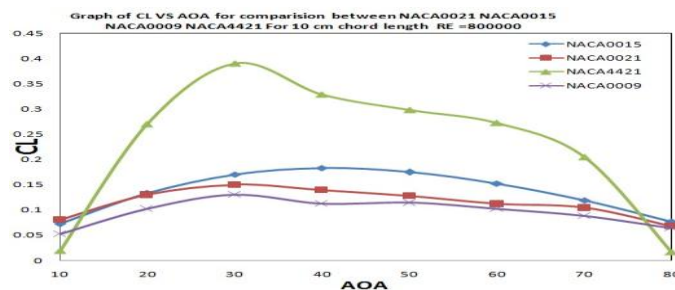
Fig.17. Graph Of CL Vs AOA For Comparison Of four blade profile for 10 cm Chord length and RE=800000
