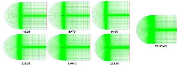
Fig.3. Grid independence study mesh
