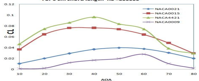
Fig. 15. Graph Of CL Vs AOA For Comparison Of four blade profile for 5 cm Chord length and RE=800000
