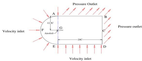
Fig. 1. Geometry with boundary conditions
