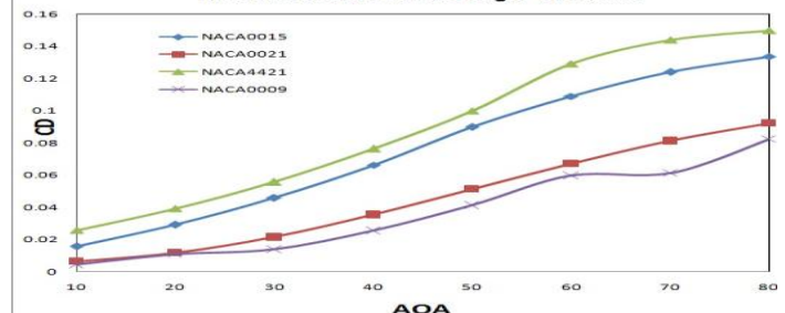
Fig. 16 Graph Of CD Vs AOA For Comparison Of four blade profile for 5 cm Chord length and RE=10000
