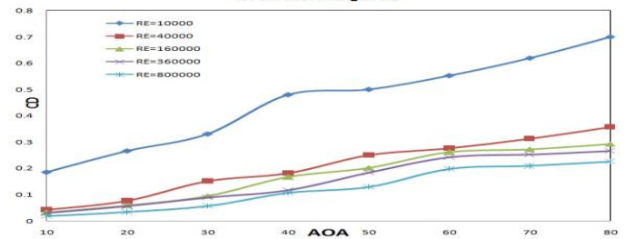
Fig. 14. Graph Of CD Vs AOA For Comparison Of Re For Naca04421 -15 Cm Chord Length
