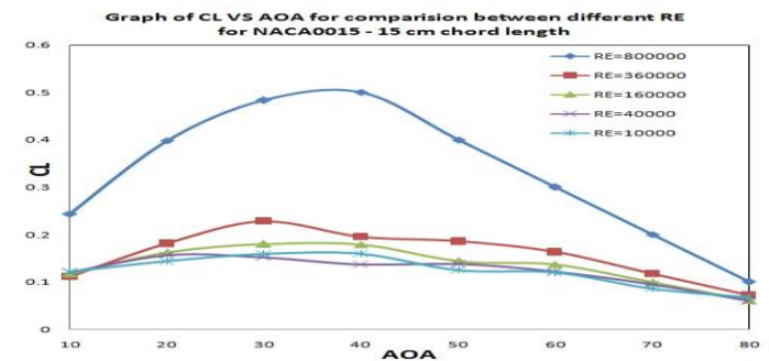
Fig.9. Graph Of CL Vs AOA For Comparison Of Re For Naca0015 - 15 Cm Chord Length
