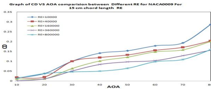
Fig. 12 Graph Of CD Vs AOA For Comparison Of Re For NACA0009 -15 Cm Chord Length
