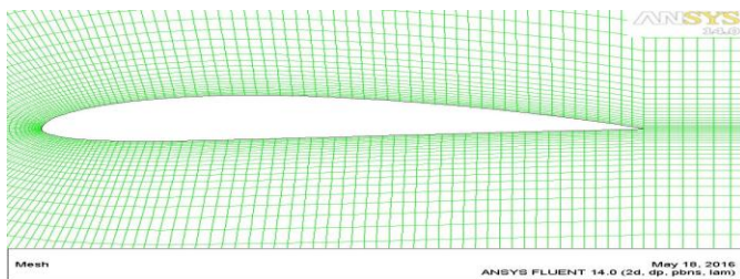
Fig. 2. Close view of C type mesh for NACA4421
