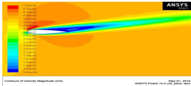
Fig.5. velocity counter for angle of attack 10^\circ
