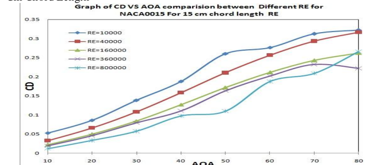
Fig.10. Graph Of CD Vs AOA For Comparison Of Re For Naca0015 - 15 Cm Chord Length
