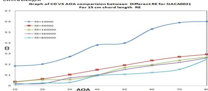
Fig. 8. Graph Of CD Vs AOA For Comparison Of Re For Naca0021 - 15 Cm Chord Length
