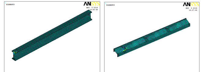
Figure 5: Meshing Models of I section and Trap Section
