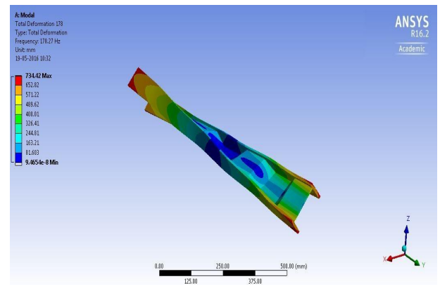
Figure 12: First Mode of trapezoidal corrugated web Beam
