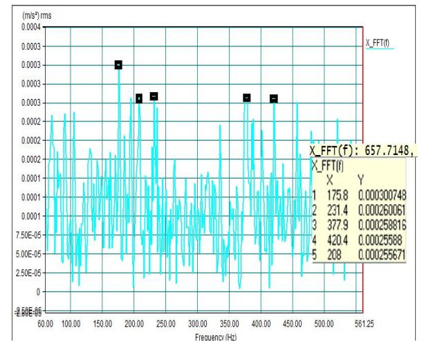
Figure 16: X Directional Waveform for I Section Beam
