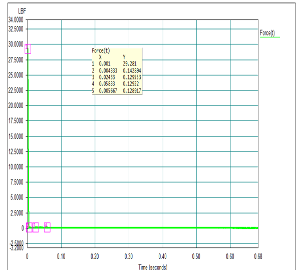
Figure 15: Load Graph for I Section Beam.
