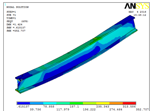
Figure 6: I section Beam Under 15 KN Loading
