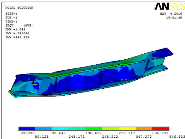
Figure 9: Trap Section Beam Under 22 kN Loading
