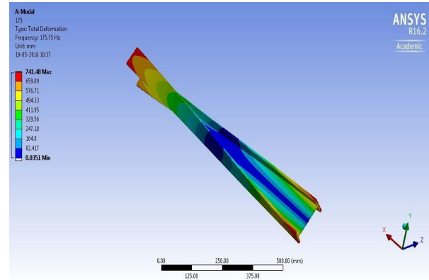
Figure 10: First Mode of I Section Beam
