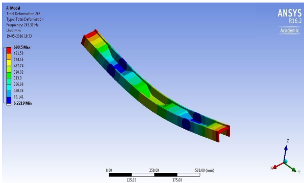
Figure 13: Second Mode of trapezoidal corrugated web Beam
