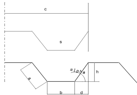
Figure 2: Trapezoidal Beam Internal Design parameters
