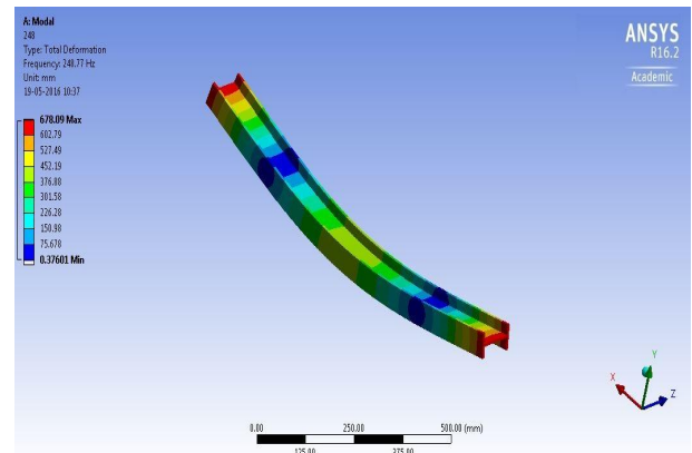
Figure 11: Second Mode of I Section Beam
