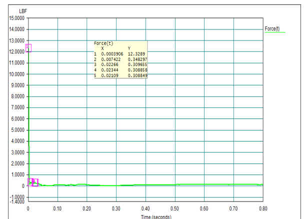
Figure 17: Load Graph for Trapezoidal Corrugated Web Beam
