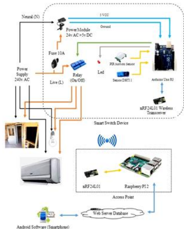
Fig. 2. System architecture
