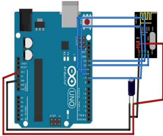
Fig. 5. nRF24L01+ Wireless Transceiver connects to Arduino UNO R3
