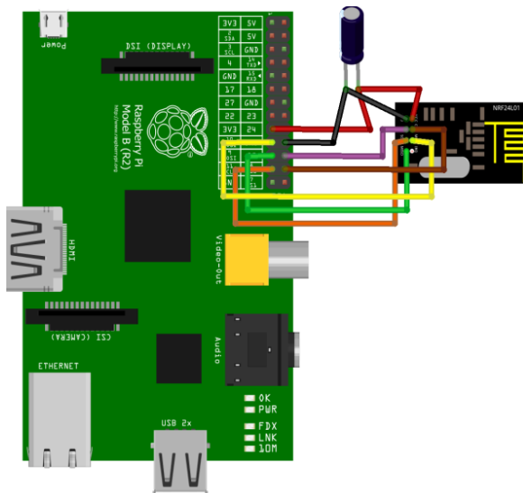
Fig. 3. nRF24L01+ Wireless Transceiver connects to Raspberry Pi 2
