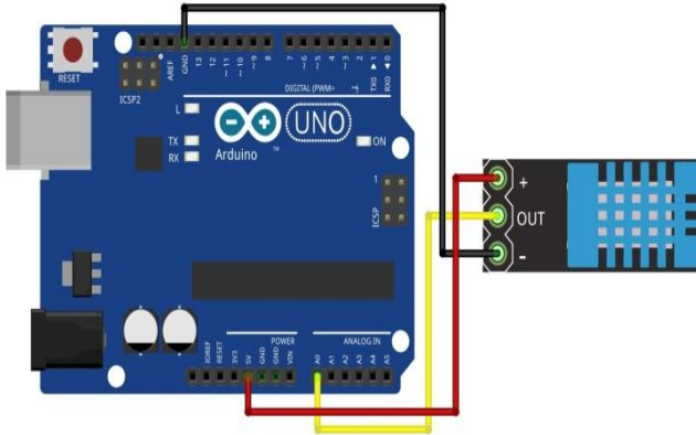
Fig. 10. Connection Circuit of Temperature and Humidity Sensor
