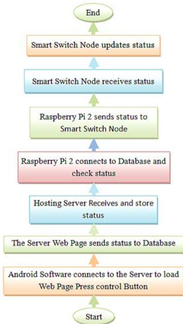
Fig. 15. Flowchart for Android app sends status to smart switch node.
