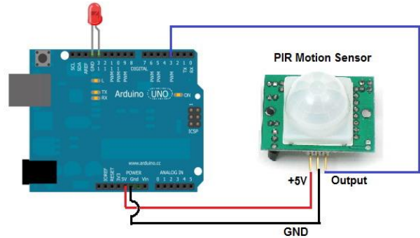
Fig. 7. Connection Circuit of PIR Motion Sensor
