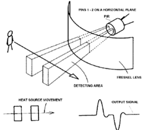
Fig. 8. The Motion Detection by PIR Sensor within the system.
