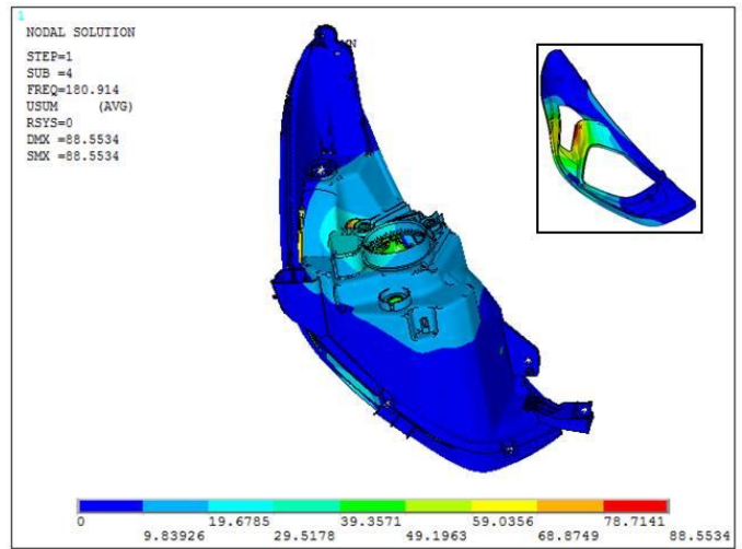
Figure 9. 4 th Mode shape of headlamp
