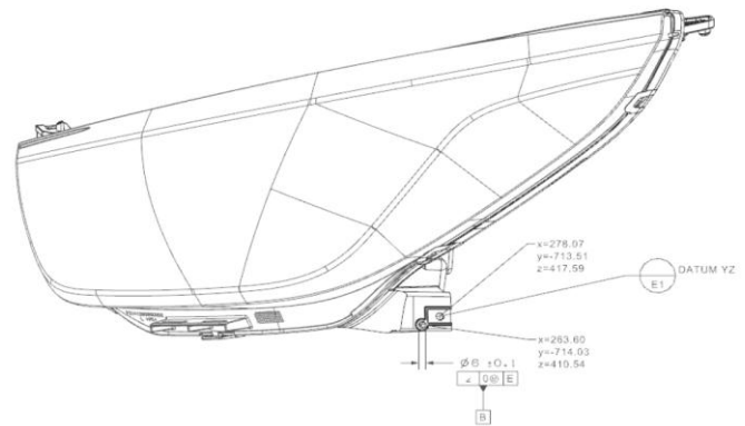
Figure 4. YZ Datum of headlamp
