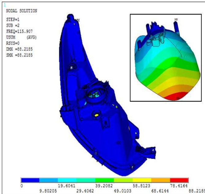
Figure 7. 2 nd Mode shape of headlamp
