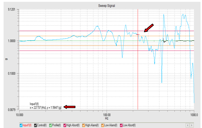
Figure 18. 6 th Mode shape of headlamp by Experimental
