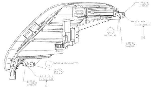
Figure 3. XYZ & YZ Datum of headlamp
