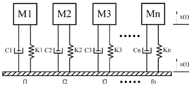
Figure 1- Shock Response Spectrum Model
