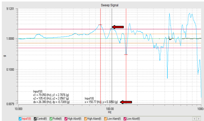
Figure 15. 3 rd Mode shape of headlamp by Experimental
