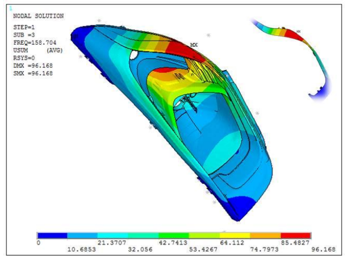
Figure 8. 3 rd Mode shape of headlamp
