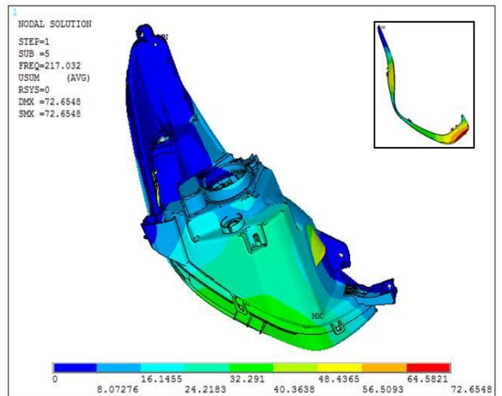
Figure 10. 5 th Mode shape of headlamp
