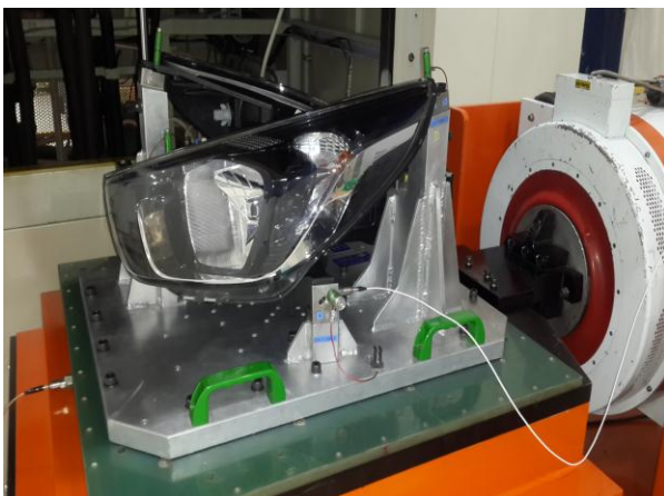
Figure 12. Experimental setup at Magneti Marelli
