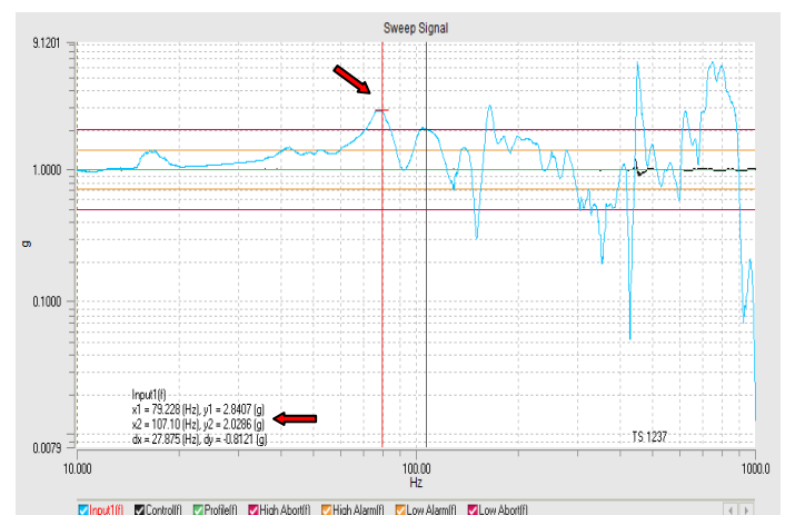
Figure 13. 1 st Mode shape of headlamp by Experimental
