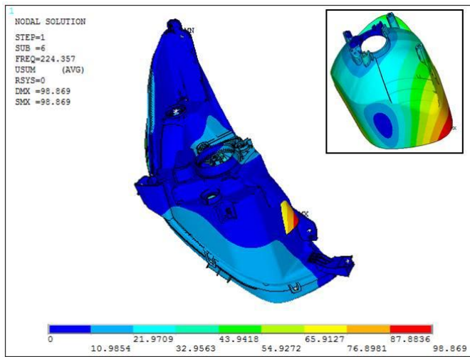
Figure 11. 6 th Mode shape of headlamp
