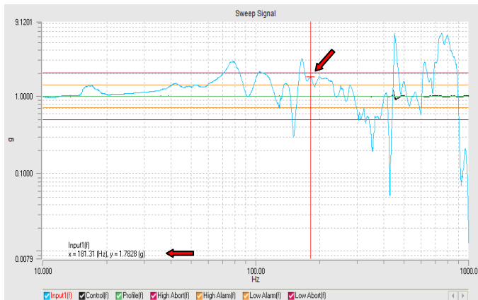
Figure 16. 4 th Mode shape of headlamp by Experimental
