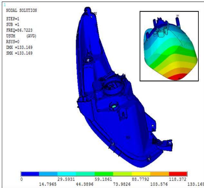
Figure 6. 1 st Mode shape of headlamp
